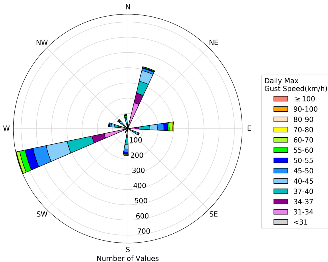
Figure 15 Daily maximum wind gust speed and direction from 1960-2019 observed at the Fort Simpson A.
